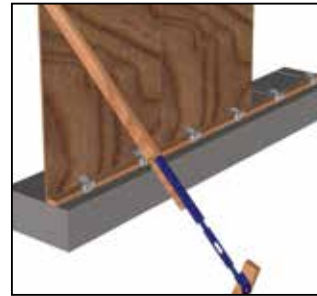
3: Nail vertical plywood panels to 2x4 kicker plate. (Or attach to inverted single waler brackets on kicker plate - support panels temporarily, as needed.)
