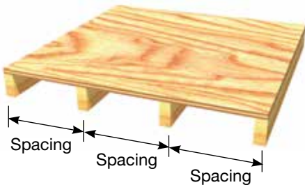
Sanded thickness, panel grain parallel to span
