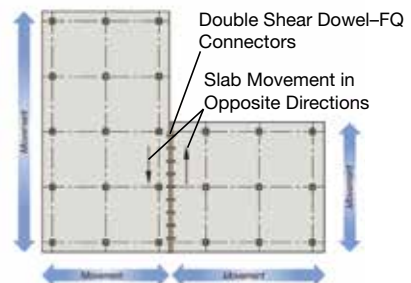
Double Shear Dowel-FQ allowing movement in two directions
